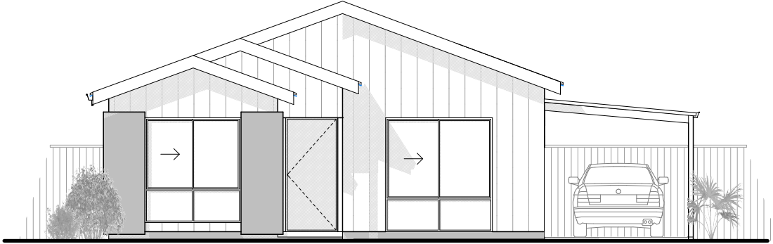
FRONT ELEVATION
